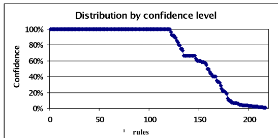
Fig. 6 Distribution of rules by Confidence Level
